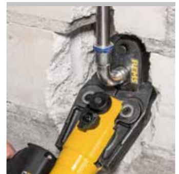
REMS pressing ring 45° (PR-2B) Patent EP 2 774 725
